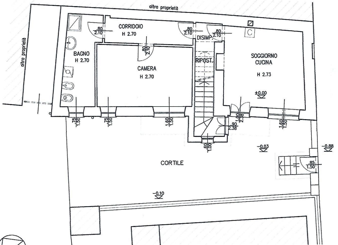
PIANO TERRA RAPP. 1:100
