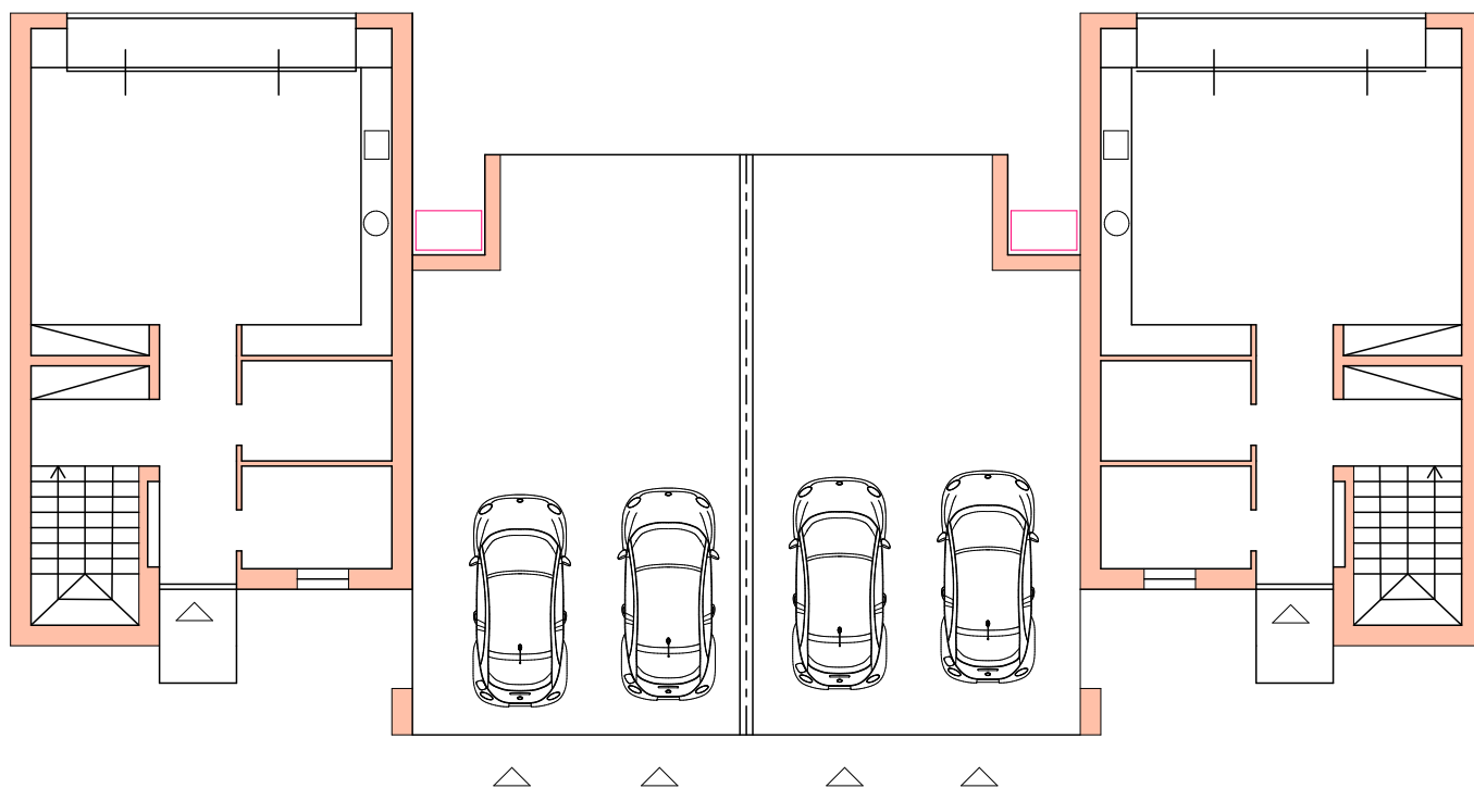
piano terra
